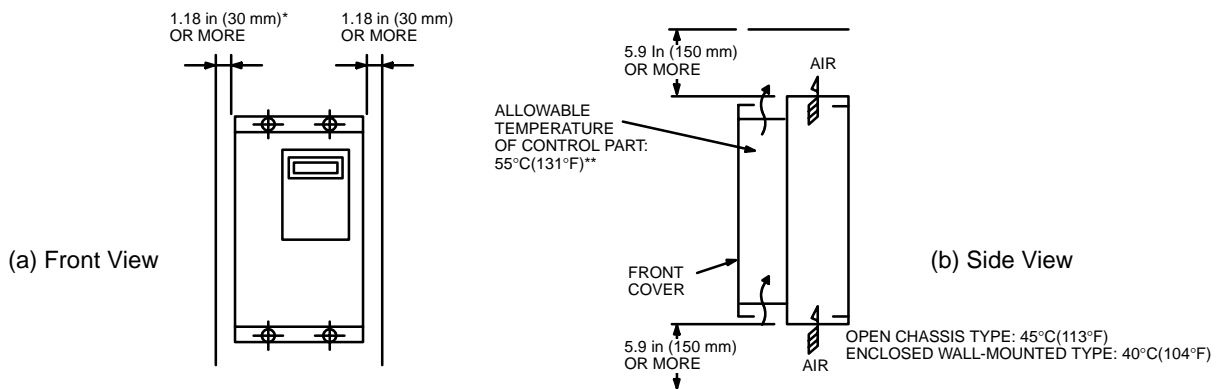
Fig. 1 Mounting Spaces
