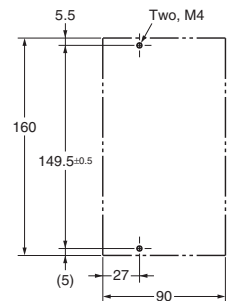
Mounting dimensions
