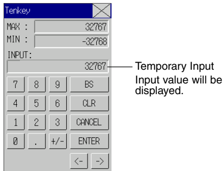
Keypad with Temporary Input
