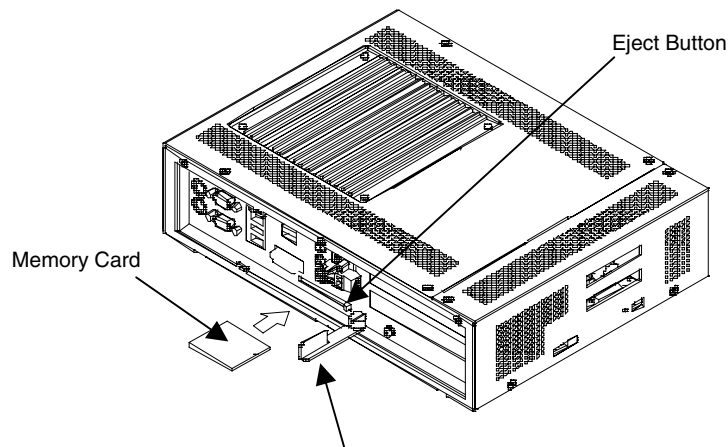
Memory Card cover (when installing or removing Card)
