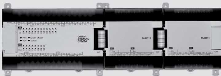
CPM2A CPU Unit with Two CPM1A-MAD11 Analogue I/O Units (2 Analogue Inputs and 1 Analogue Output)
