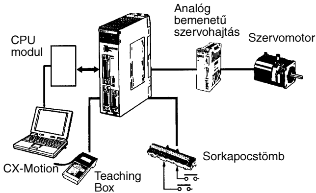
CS1W-MC421
