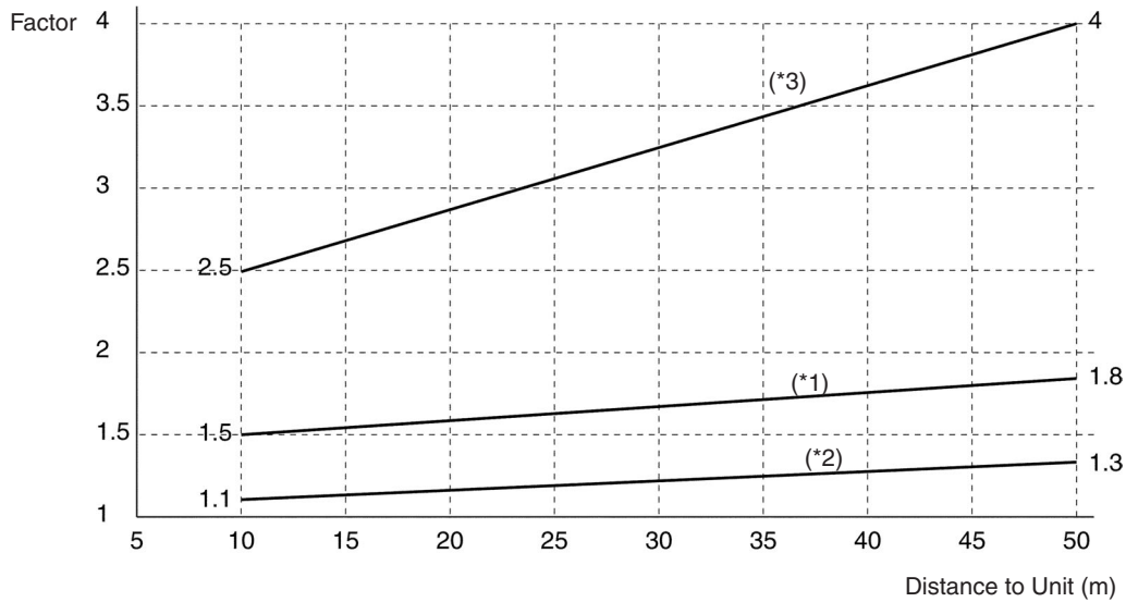
I/O Unit Refresh Time Coefficients for Units on CS-series Long-distance Expansion Racks
