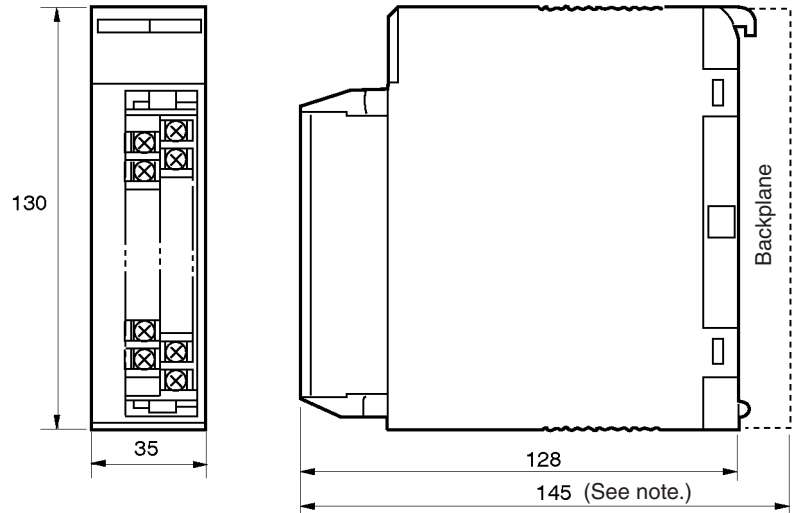
Terminal Dimensions
