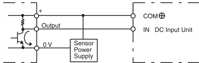
Voltage output
