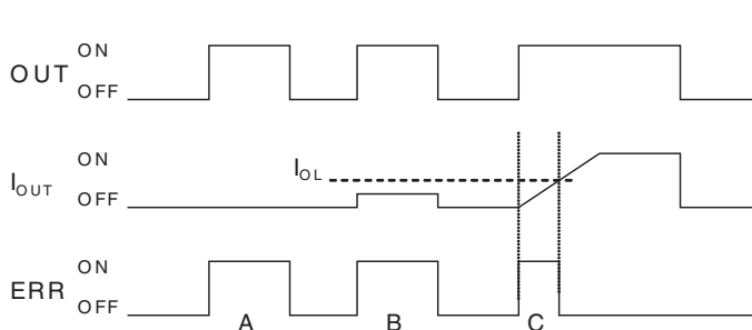
Figure 3: Line Disconnections
