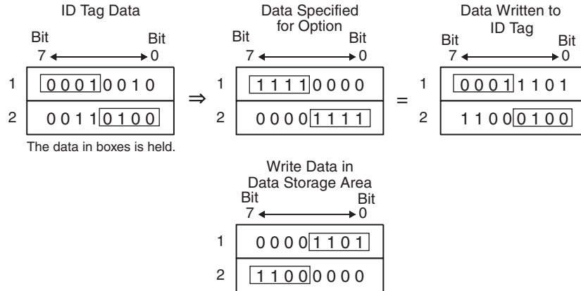
Example for a Masked Bit Write
