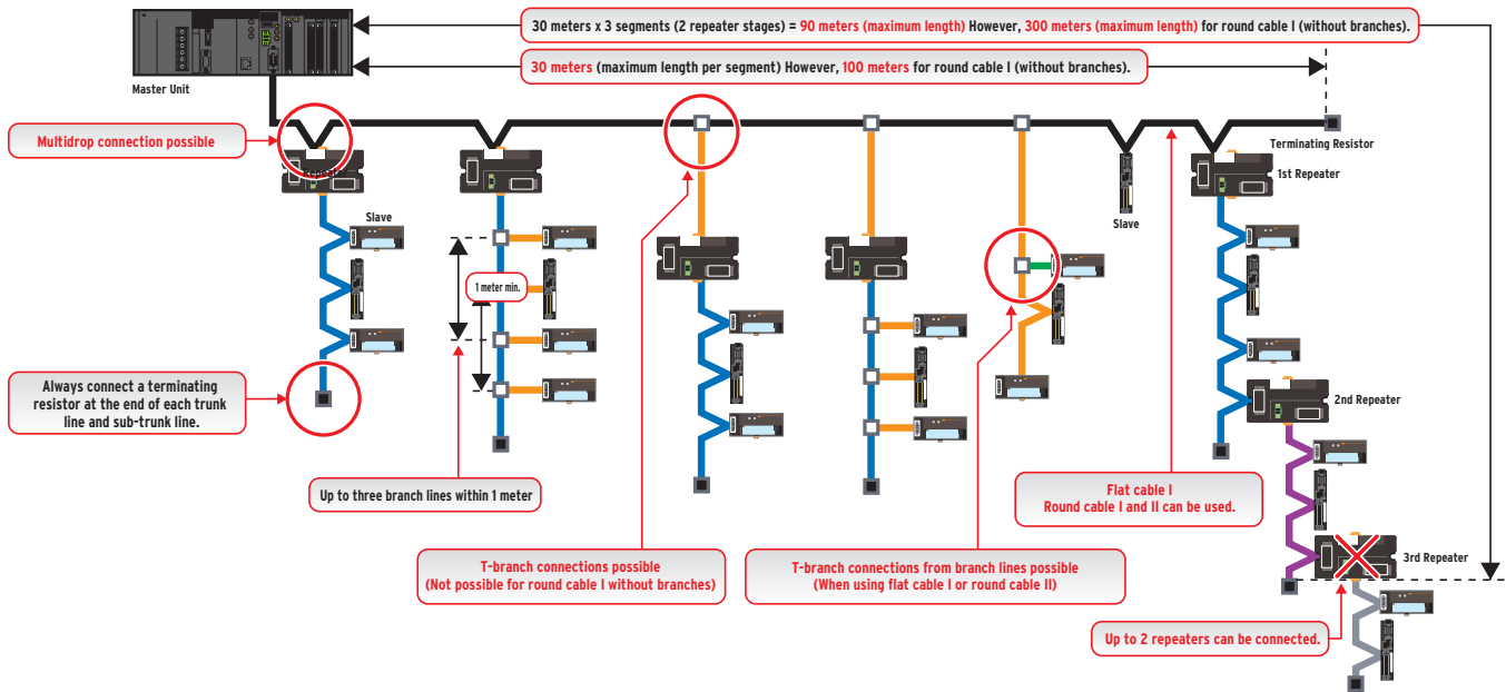
Example of wiring for 1.5 Mbps (Application: Balance of fast communications and branching)
