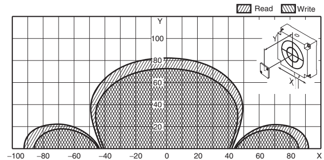
V680-HS63 (mounted on non-metallic material) & V680-D1KP66T-SP
