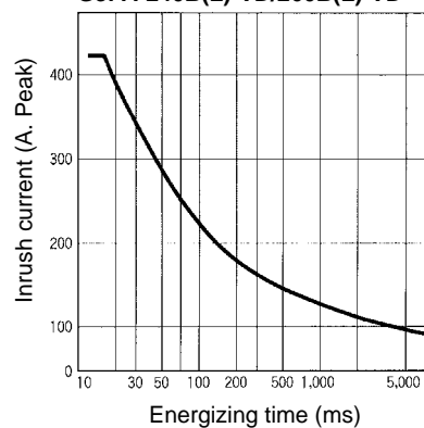
G3PA-240B(L)-VD/260B(L)-VD
