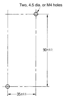
Mounting Holes
