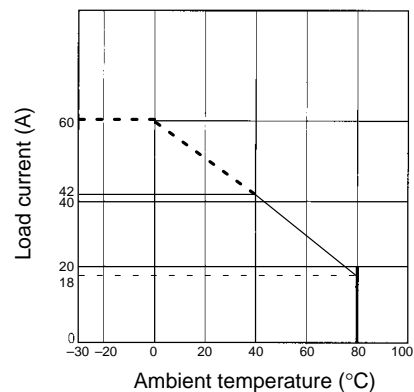
G3PA-260B(L)-VD
