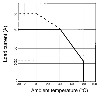
G3PA-260B(L)-VD
