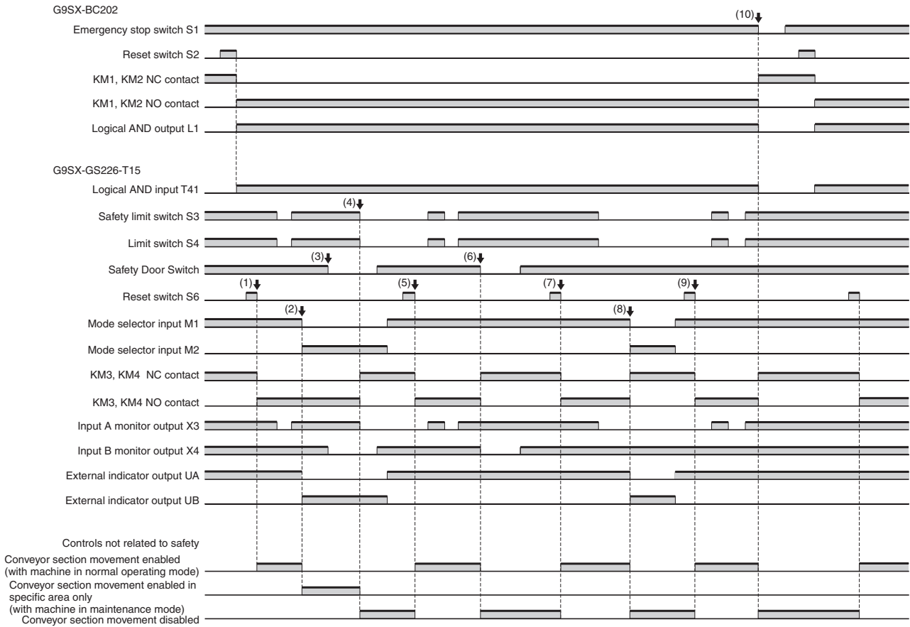
Timing Chart 2
