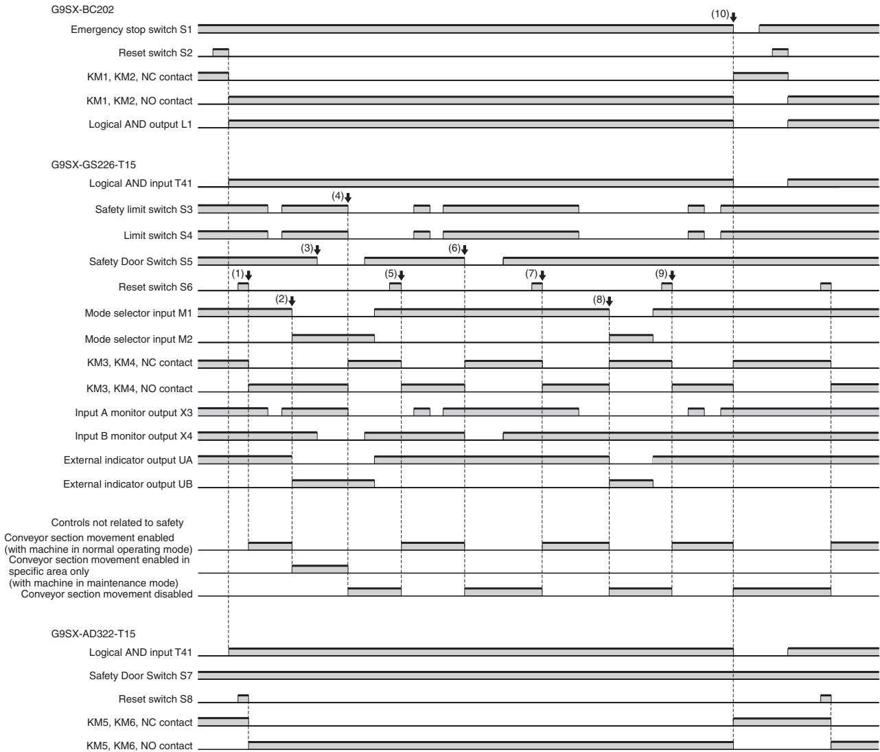
Timing Chart 3
